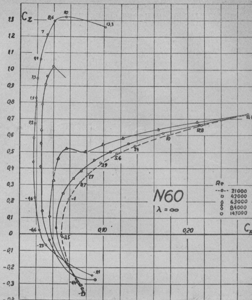
Krzywe profili N 60 i 417a
